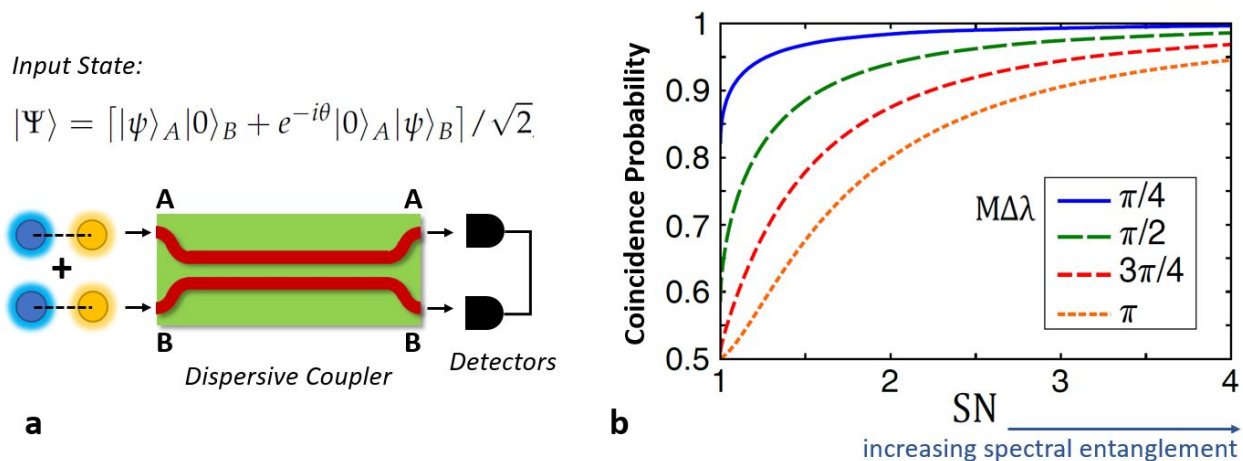
Figure 1: Influence of coupler dispersion and state properties on time-reversed HOM interference; (a) input conditions; (b) probability of obtaining a coincidence count (separated outcome) at the coupler output [4].
