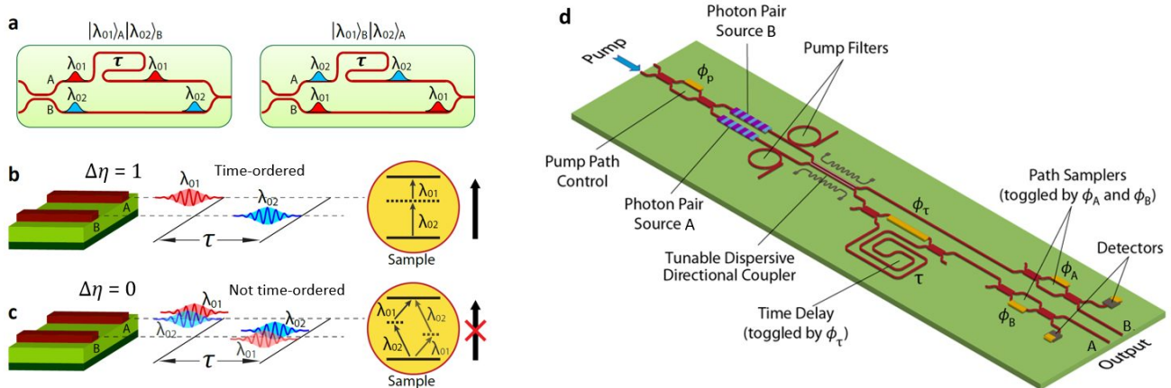
Figure 3: (a-c) Dispersion-enabled control over photon time ordering; (d) example of a monolithic photonic quantum circuit where a single dispersive coupler provides multiple functionalities (see text) [4].
