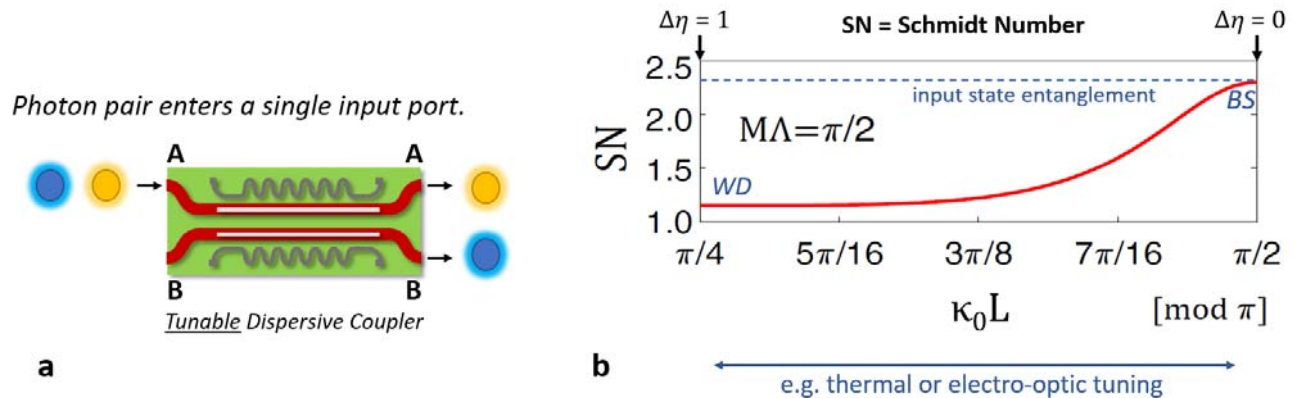
Figure 2: Dispersion-enabled control over spectral entanglement; (a) implementation; (b) dependence of output entanglement on coupler response, where \Lambda = |\lambda_{02} - \lambda_{01}| is the photon pair non-degeneracy and \kappa_0 is the coupling strength at an arbitrary reference wavelength [4].
